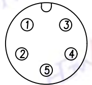
HGF02-M805P-CB
